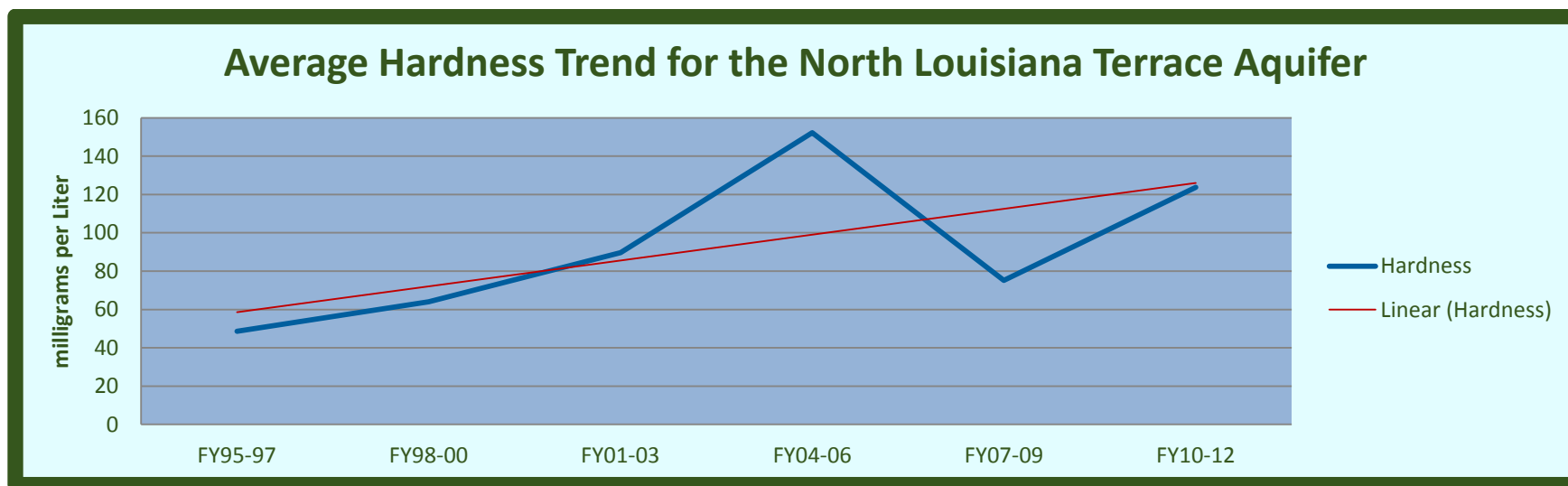
Chart 6-12: Hardness Trend
