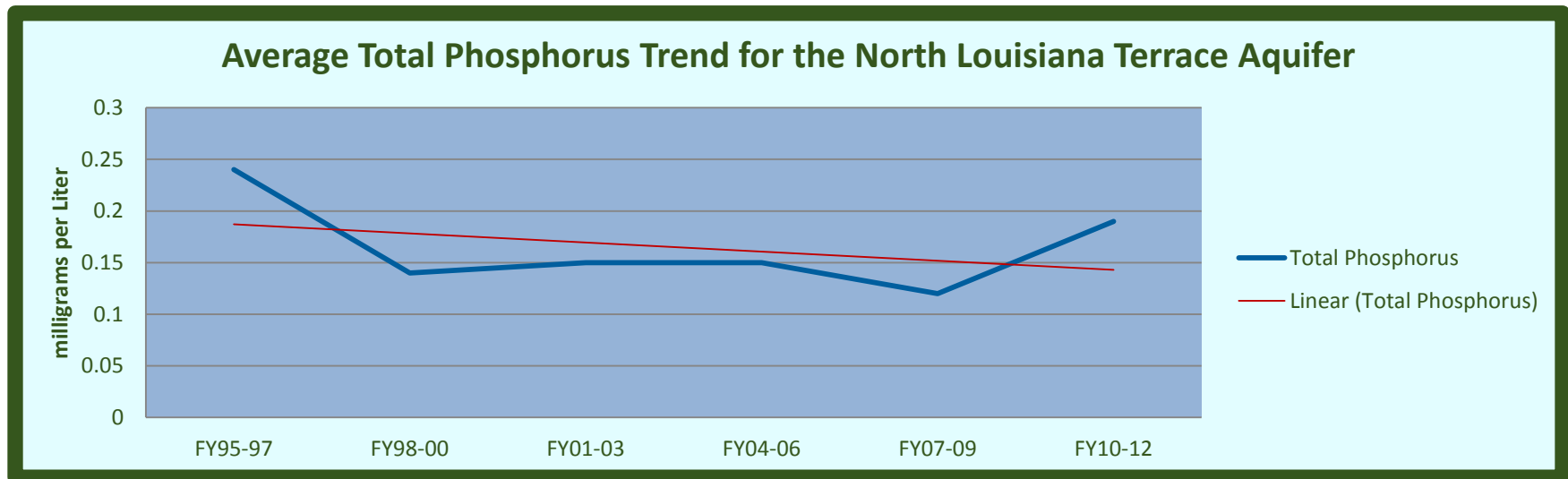
Chart 6-15: Total Phosphorus Trend
