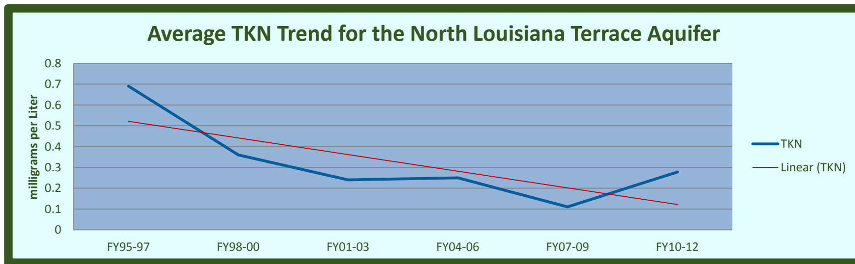
Chart 6-14: TKN Trend
